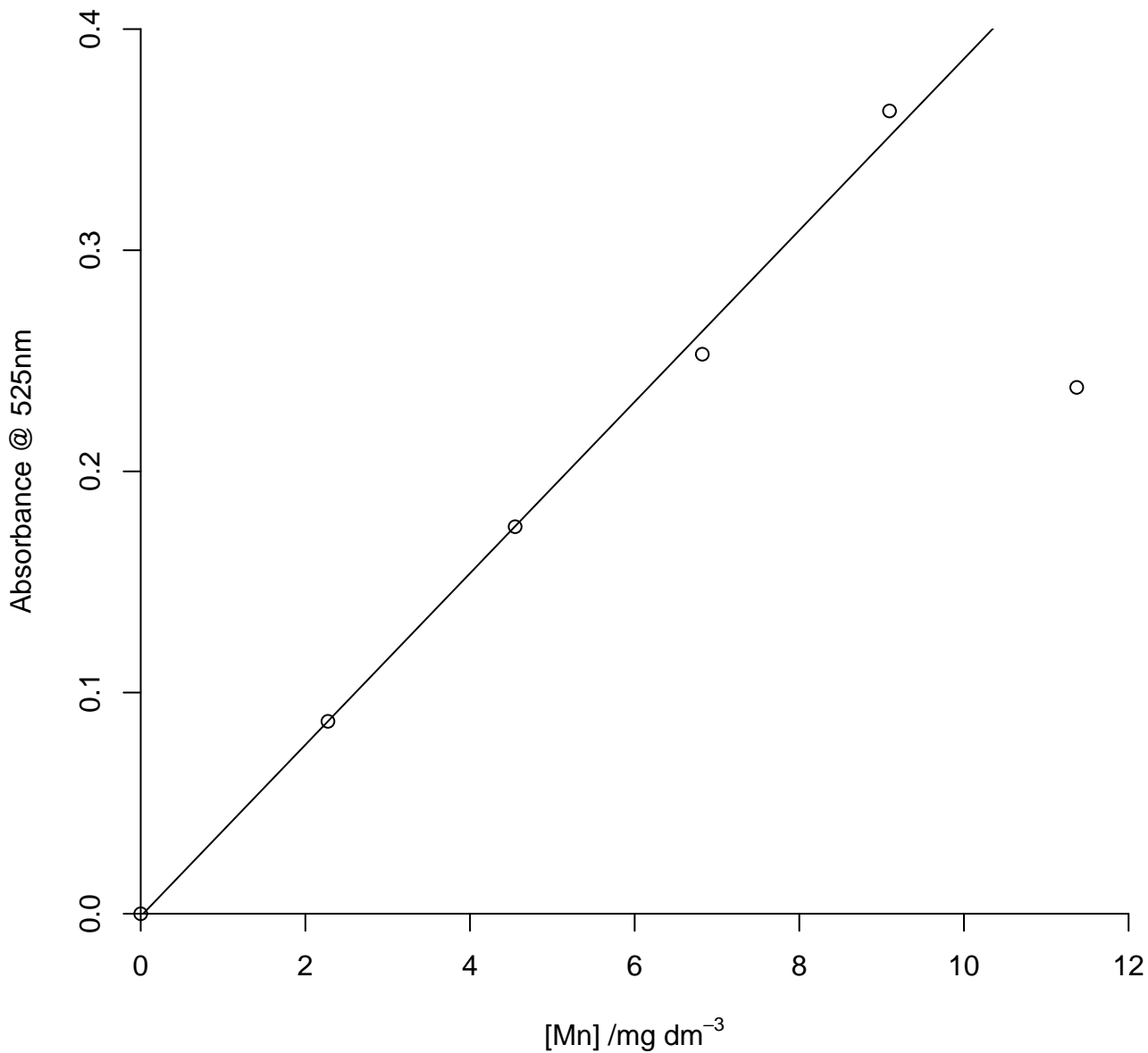
Calibration graph for \text{KMnO}_4
